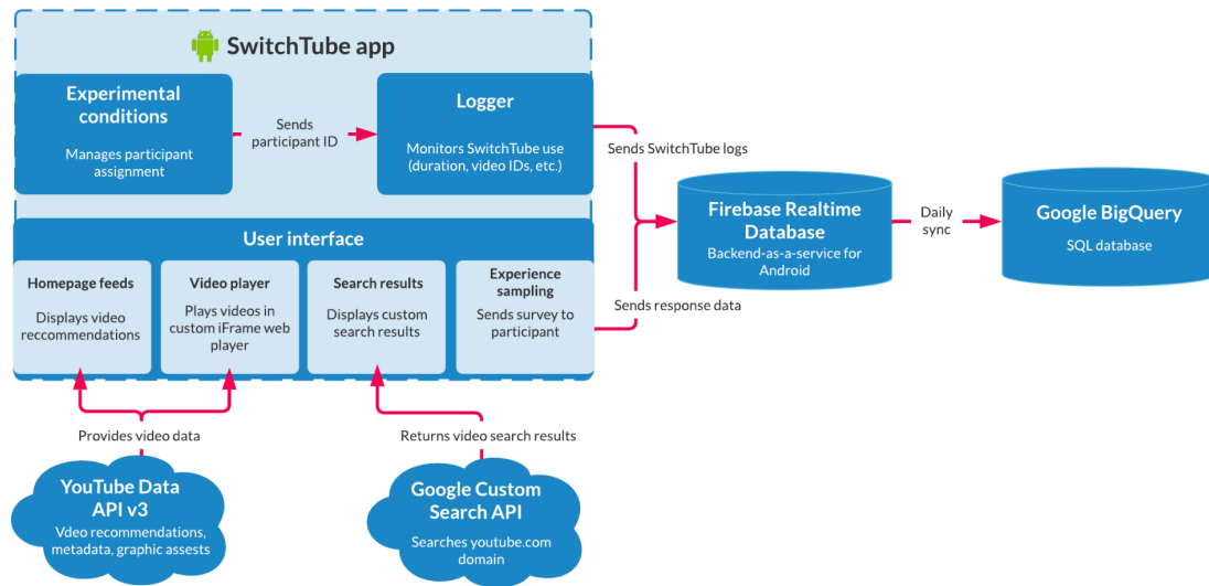
Figure 19. The technical implementation of the SwitchTube study app for Android.
