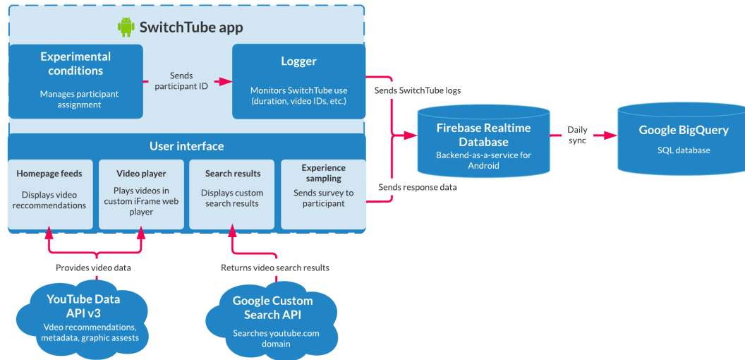
Fig. 6. The technical implementation of the SwitchTube study app for Android.
