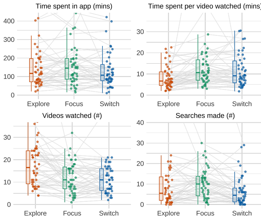
Fig. 7. Log data from our deployment study with 46 participants for the three versions of the SwitchTube app: Explore, Focus, and Switch. Participants spent more time in Focus than Explore. Participants also spent more time on each video that they watched (or started) in Focus, although they actually watched more videos in Explore. Participants in Focus also made more searches than in the other versions. For a detailed explanation of the format used for this figure, which is repeated in several subsequent figures, see the footnote. 5
